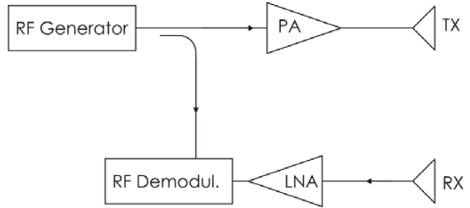
Fig. 3 - Coherent CW RADAR
